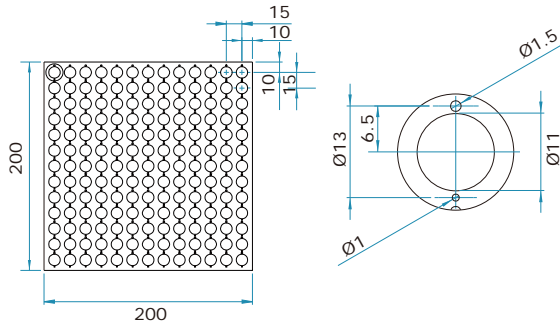
optical panel(OP-100-01)/rear
