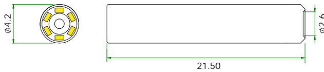
Tube type
